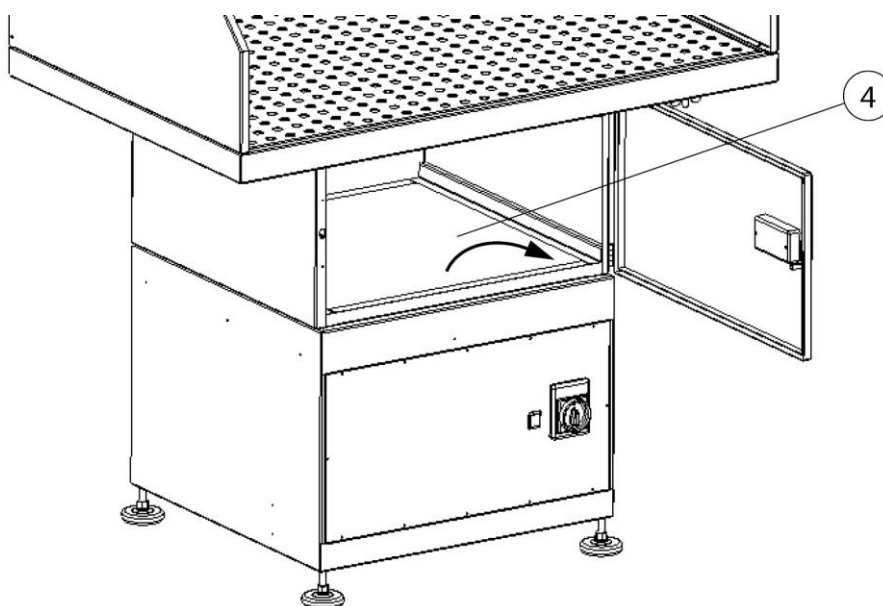
Fig. 11: Filter change – activated charcoal filter (optional)
