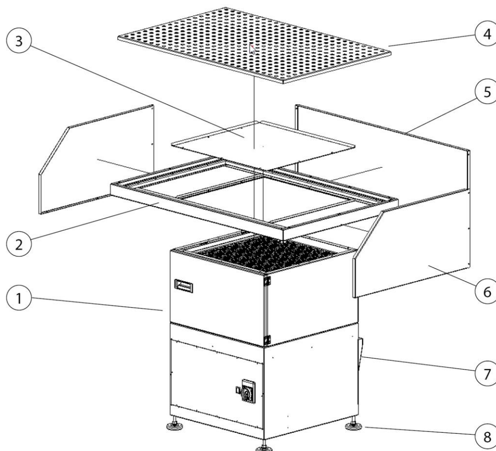
Fig. 2: Assembly
